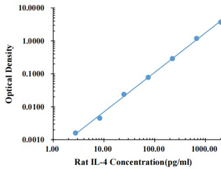
Rat IL-4 Typical Standard
